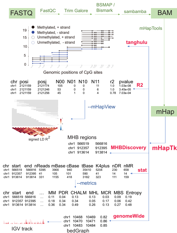
Fig. 1. A schematic diagram of mHapTk. The pre-processing steps output mHap files that are used as standard input in mHapTk. There are five sub-commands in mHapTk, including 'tanghulu', 'R2', 'MHBDiscovery', 'stat' and 'genomeWide'. The example outputs of each command are shown in a concise way
